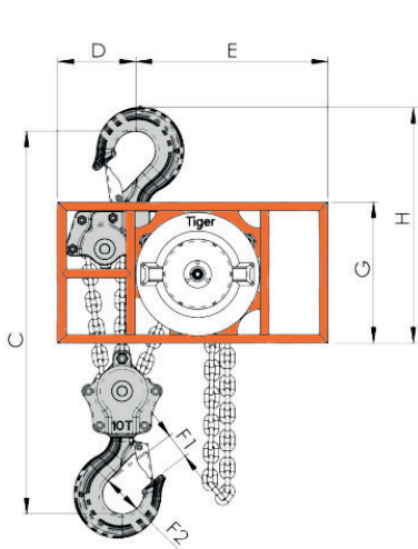
10t rotary torque
