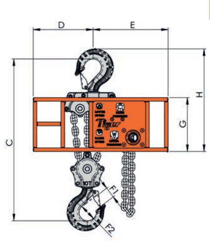
10t hot stab
