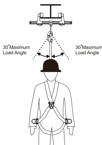
Trolley Load Angle
