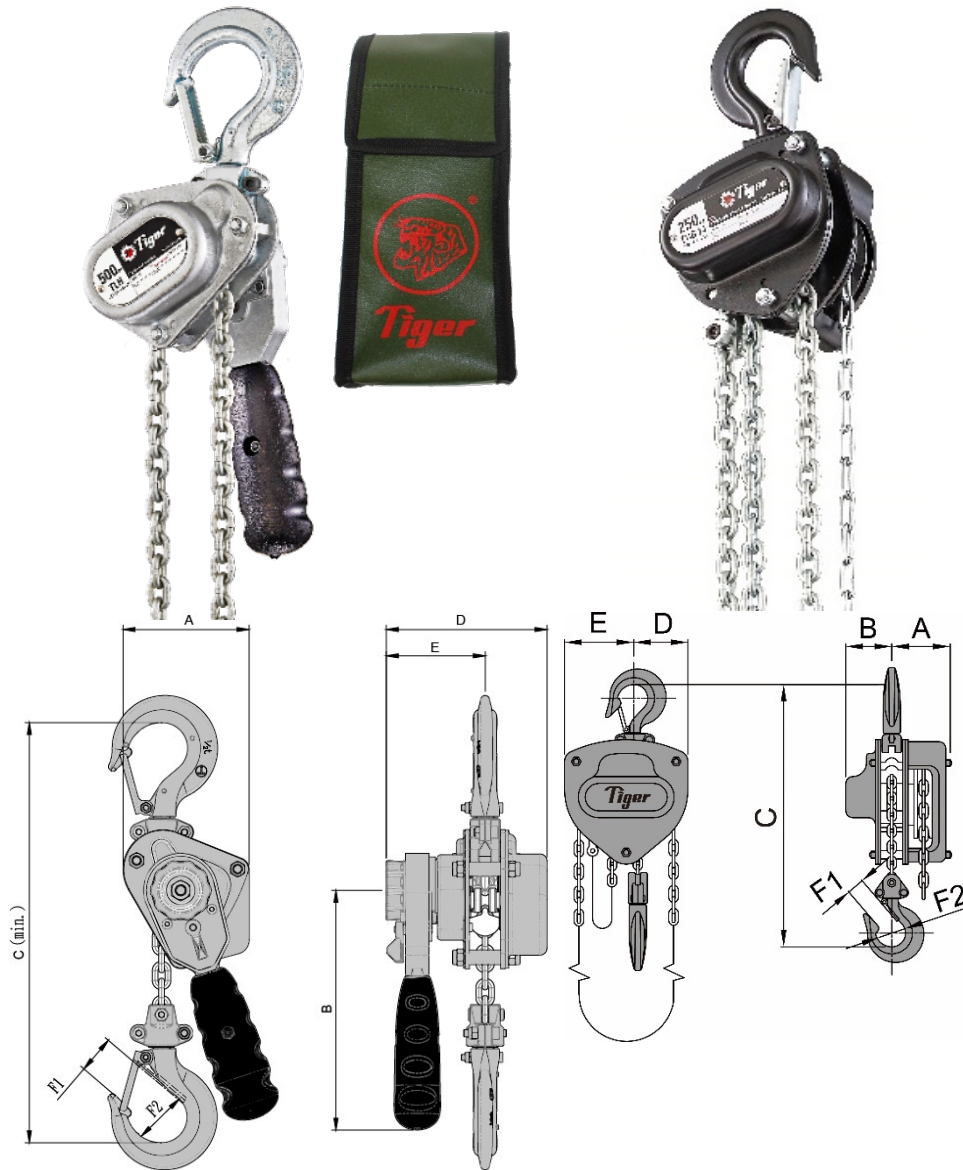
0.25t (LH-0025) & 0.5t lever hoist (LH-0050)
